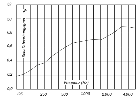
Sound absorption level – octave centre frequency
