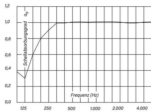
Broadband-Wall-Absorber 90
